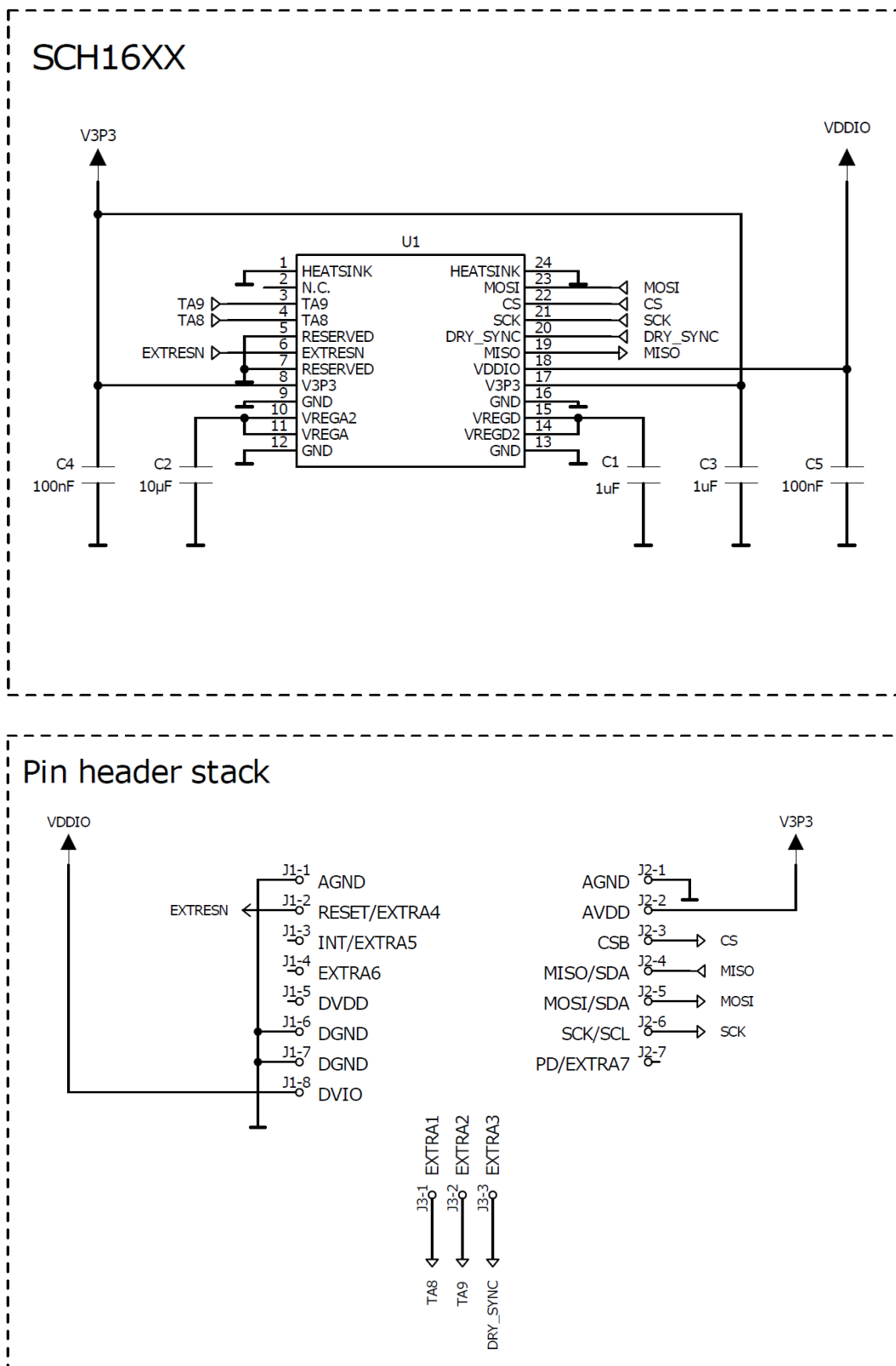
Figure 4. SCH1600 PCB circuit diagram
